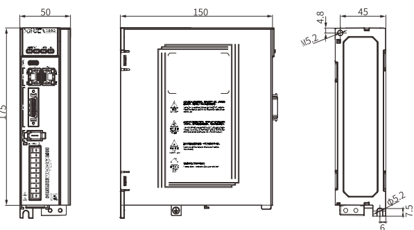
DS6C-20P7
