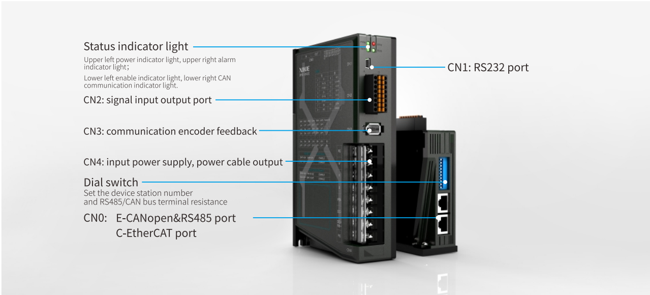
CN2 port (taking DF3E-0410 as an example)
