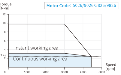
MS6S-100CM/TL30B(Z)2-21P0
