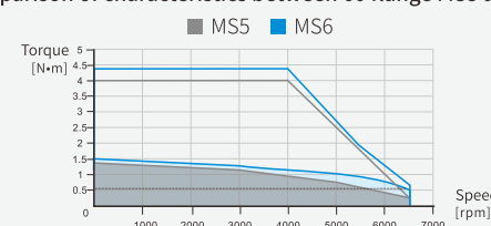
Comparison of characteristics between 60 flange MS5 and MS6
