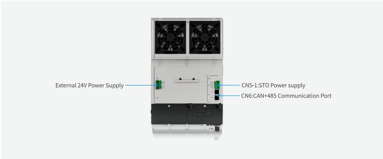
DM6C-44P0S/455P0S/475P0S-M Inverter module top view terminal layout
