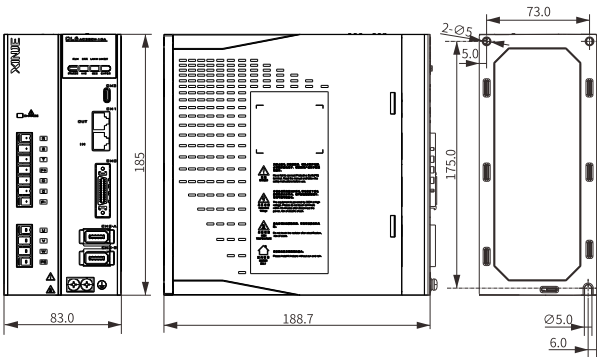
DL6-4010/4012
