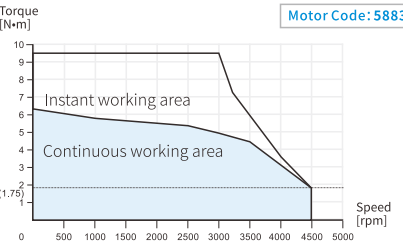
MS6S-100CM30BZ2-21P5
