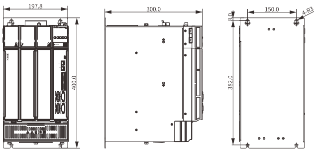
DM6C-445P0/455P0S/475P0S-M
